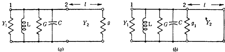
FIG. 14-13.—Equivalent circuits for double-output tuning.
